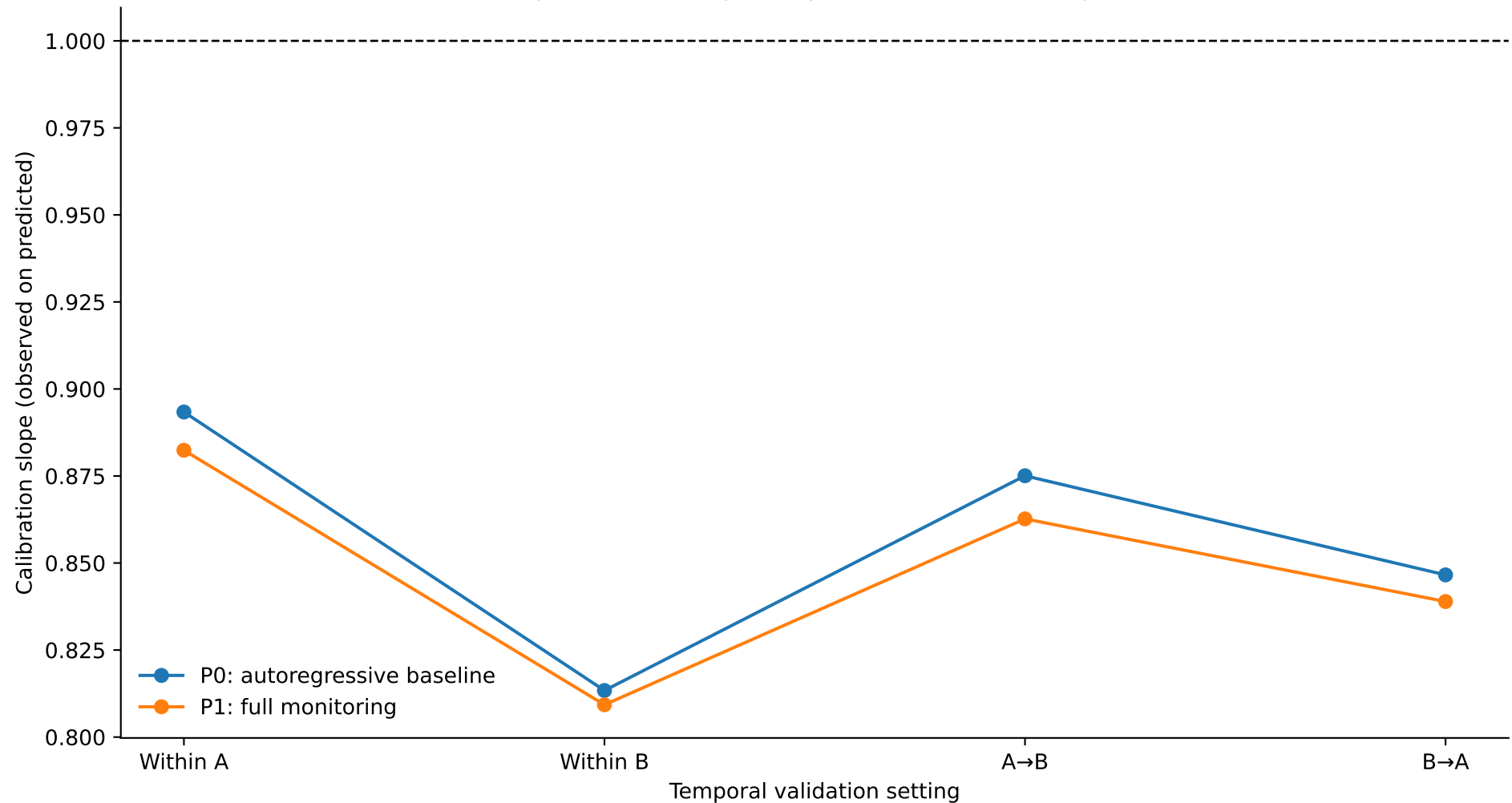
Calibration slopes under the primary 28-observation adaptation window
