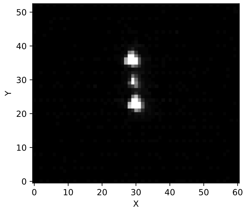
STACK + PSF
