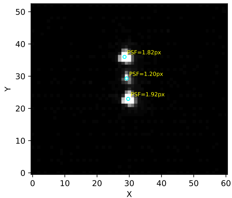
STACK + PSF
