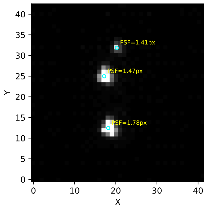
STACK + PSF
