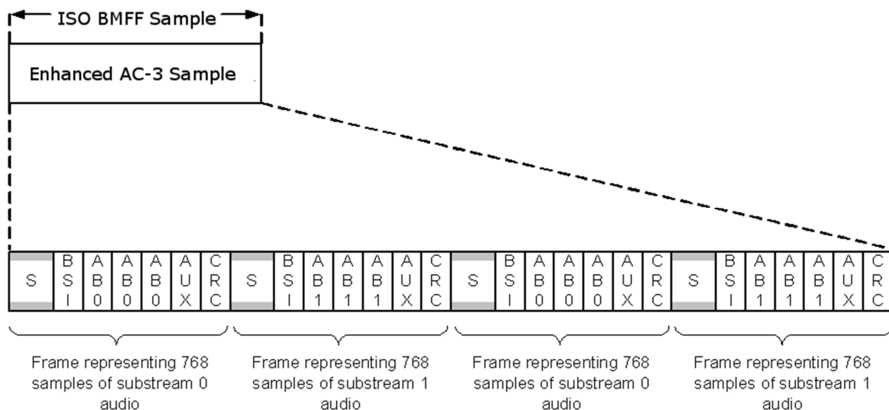
Figure F.2.3: ISO BMFF sample with two substreams with three blocks per frame
