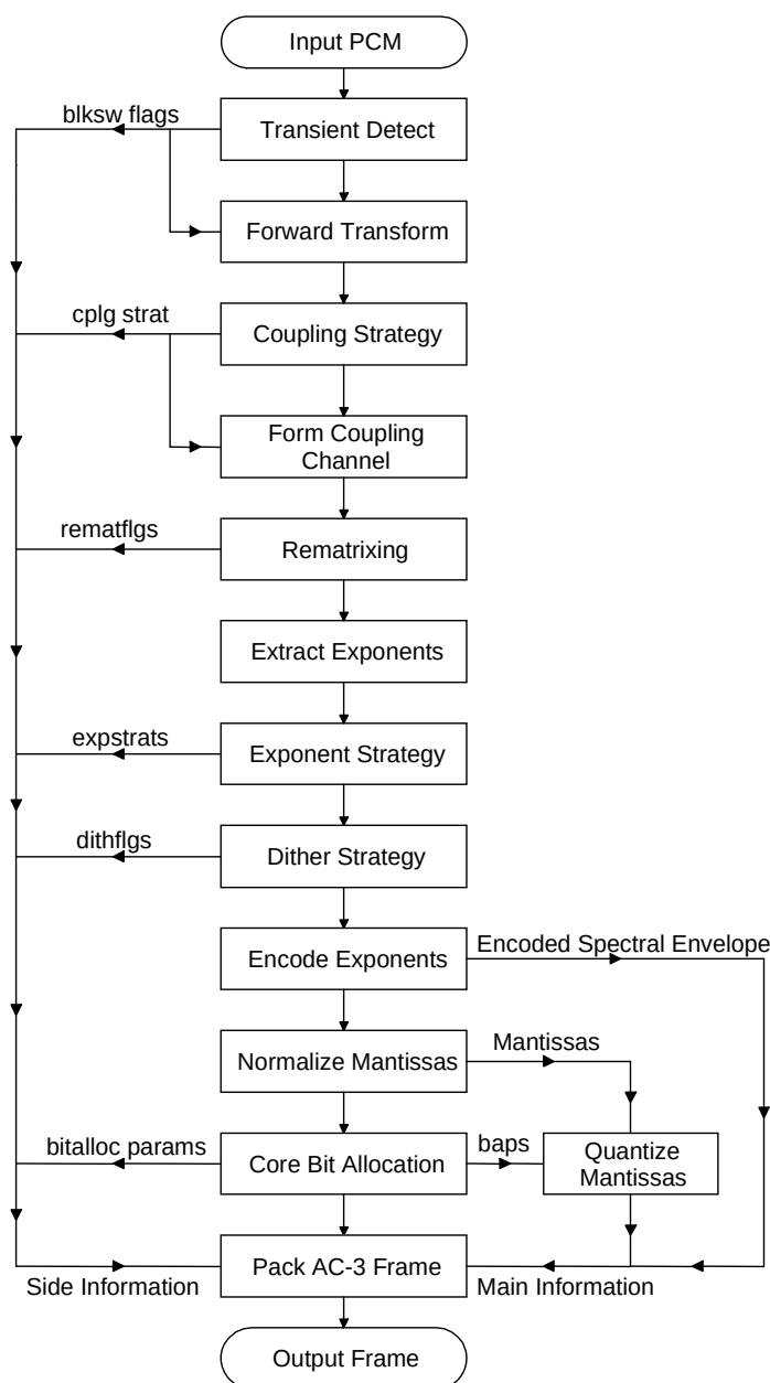
Figure 7.1: Flow diagram of the encoding process
