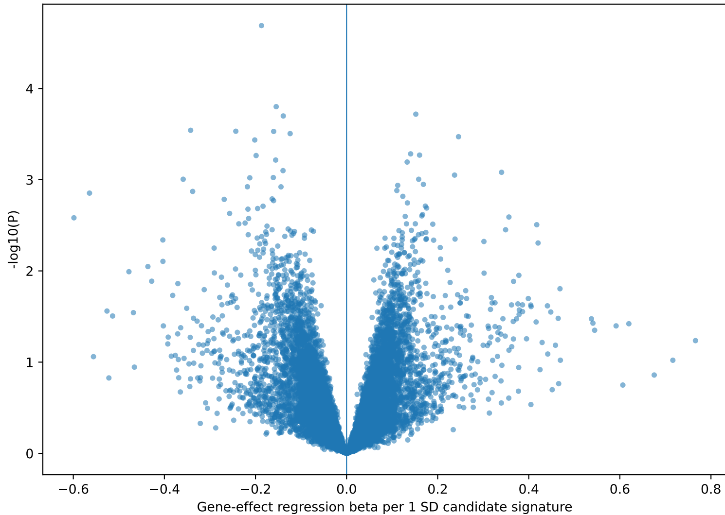
DepMap genome-wide CRISPR dependency screen
