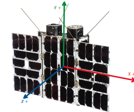
Figure 7.1.1: 6U spacecraft body frame definition used for both simulators. Courtesy of [26]
