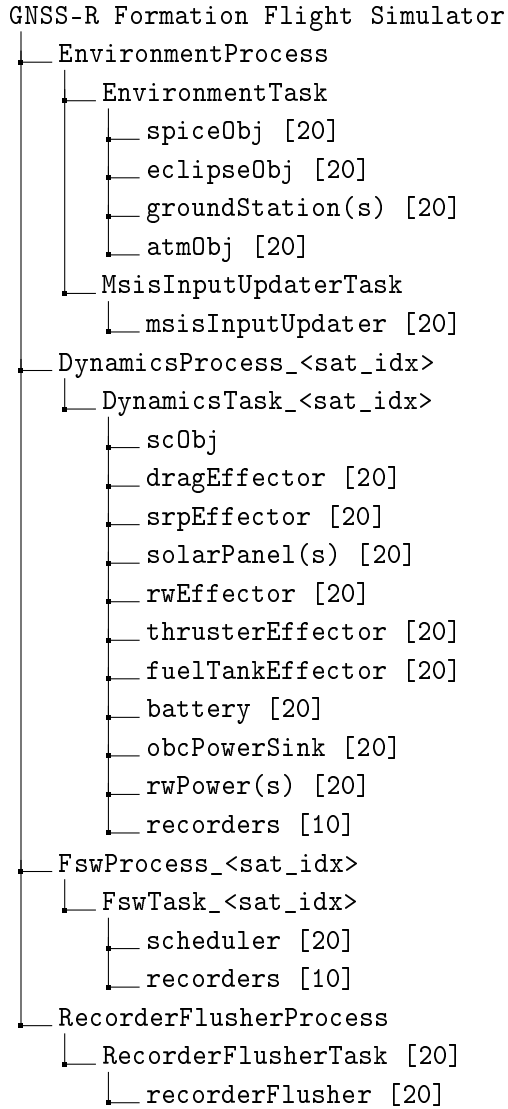
Figure 6.5.1: Hierarchical process-task-model structure of the GNSS-R formation flight Basilisk simulator. The number in square brackets denote the model priority, where higher priority models are updated first. Same-priority tasks are orderly updated from the top-down within a task. " <sat_idx> " represent per-spacecraft processes and tasks.
