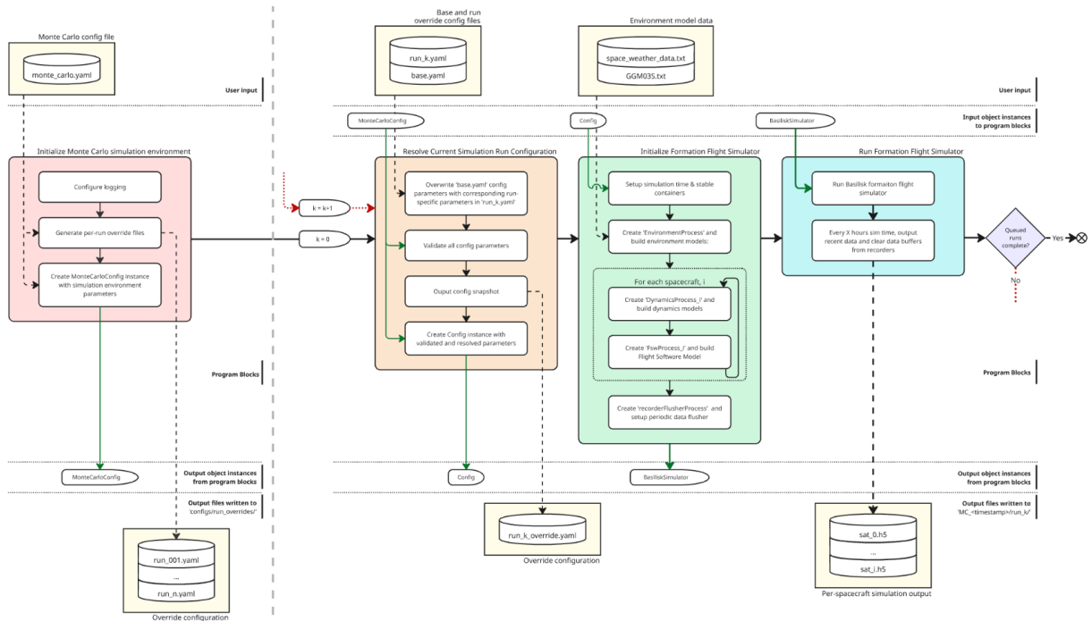
Figure 6.1.2: Detailed GNSS-R formation flight simulator flow diagram. A full-size version of this diagram is shown in the Appendix Figure B.2.1
