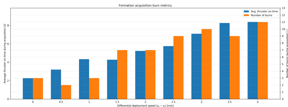
Figure F.1.1: Burn statistics for every case in the differential deployment speed fuel sensitivity campaign. The blue column shows the average duration each burn lasted, while the orange column shows the number of insertion/maintenance burns
