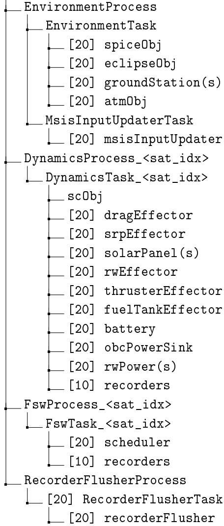
Figure D.2.1: TODO: Update and verify after simulator update. Hierarchical process-task-model structure of the GNSS-R formation flight Basilisk simulator. The number in square brackets denote the model priority, where higher priority models are updated first. Same-priority tasks are orderly updated from the top-down within a task. “<sat_idx>” represents per-spacecraft processes and tasks.
