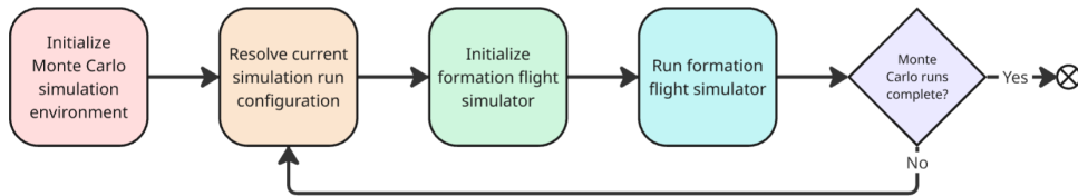
Figure 6.1.1: Simplified GNSS-R formation flight simulator flow diagram
