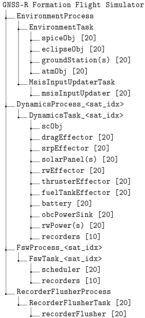
Figure 6.4.1: Hierarchical process-task-model structure of the GNSS-R formation flight Basilisk simulator. The number in square brackets denote the model priority, where higher priority models are updated first. Same-priority tasks are orderly updated from the top-down within a task. " <sat_idx> " represent per-spacecraft processes and tasks.
