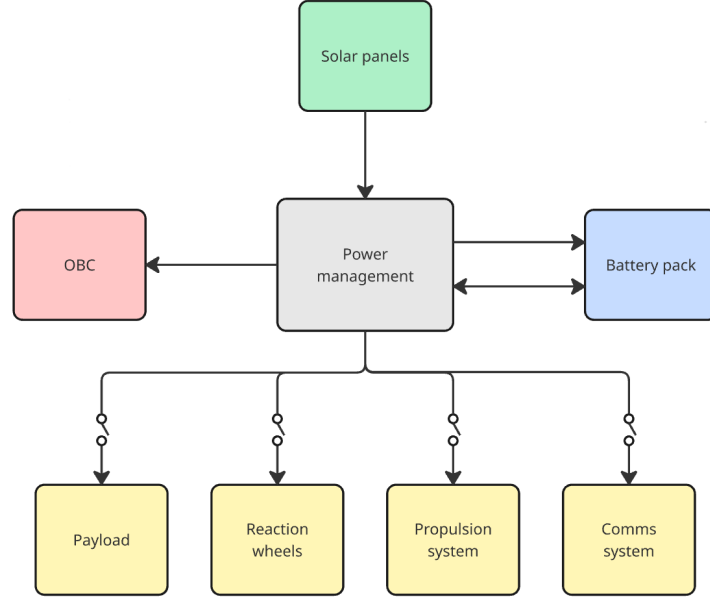
Figure 6.2.1: Overview of the per-spacecraft EPS
