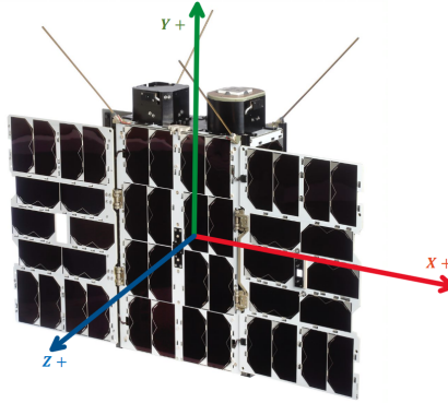
Figure 5.1.1: 6U spacecraft body frame definition used for both simulators. Courtesy of [26]
