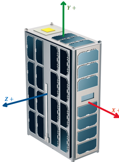
Figure 5.1.2: 6U spacecraft body frame definition used for both simulators. Adopted from [27]
