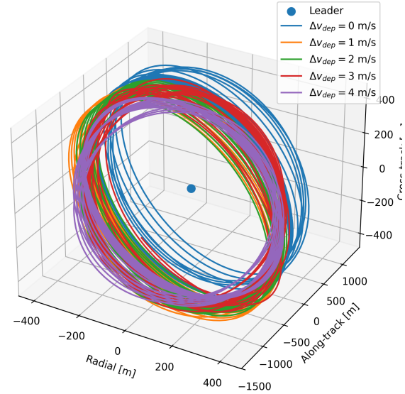
Leader-follower RTN relative-position trajectories, t \in [15, 48] h
