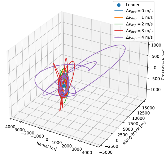
Leader-follower RTN relative-position trajectories, t \in [0, 15] h
