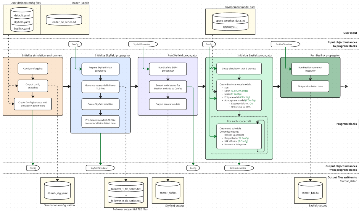
Figure 5.1.1: Detailed Comparative Propagation Simulator flow diagram. Adopted from [4]
