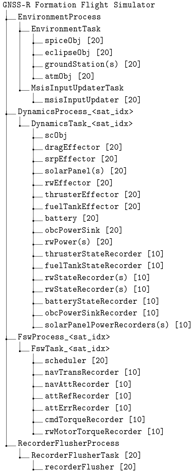
Figure 6.4.1: Hierarchical process-task-model structure of the GNSS-R formation flight Basilisk simulator. The number in square brackets denote the model priority, where higher priority models are updated first. Same-priority tasks are orderly updated from the top-down within a task. " <sat_idx> " represent per-spacecraft processes and tasks.
