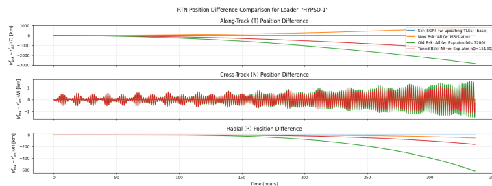
Figure 9.1.2: Decomposition of the same-spacecraft position difference in the RTN frame
