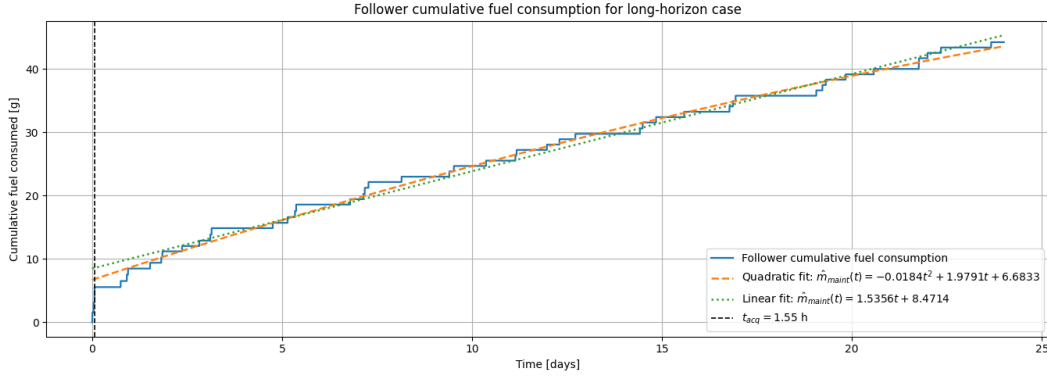
Figure 9.3.1: Cumulative fuel consumption for a zero differential deployment speed case over 24 days. A quadratic and linear model has been fitted to the cumulative fuel consumption using samples in the timespan t \in [t_{\text{acq}}, t_{\text{end}}]
