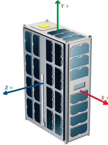
Figure 7.1.1: 6U spacecraft body frame definition used for both simulators. Adopted from [38]
