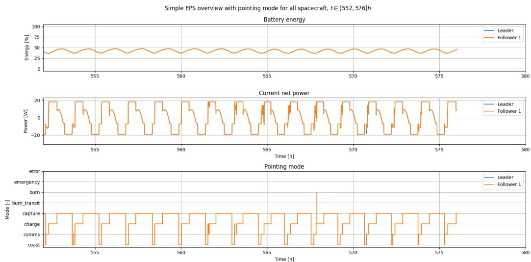
Figure 9.3.2: Operational mode transitions and EPS parameters for the leader and follower spacecraft during the final hours of the steady-state campaign
