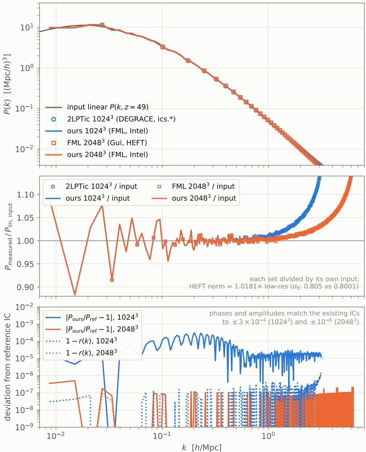
IC power spectra: our Intel-built 2LPTIC (FML) vs existing DEGRACE / HEFT ICs L = 1024 \text{ Mpc}/h , z_{\text{ini}} = 49 , seed 2026
