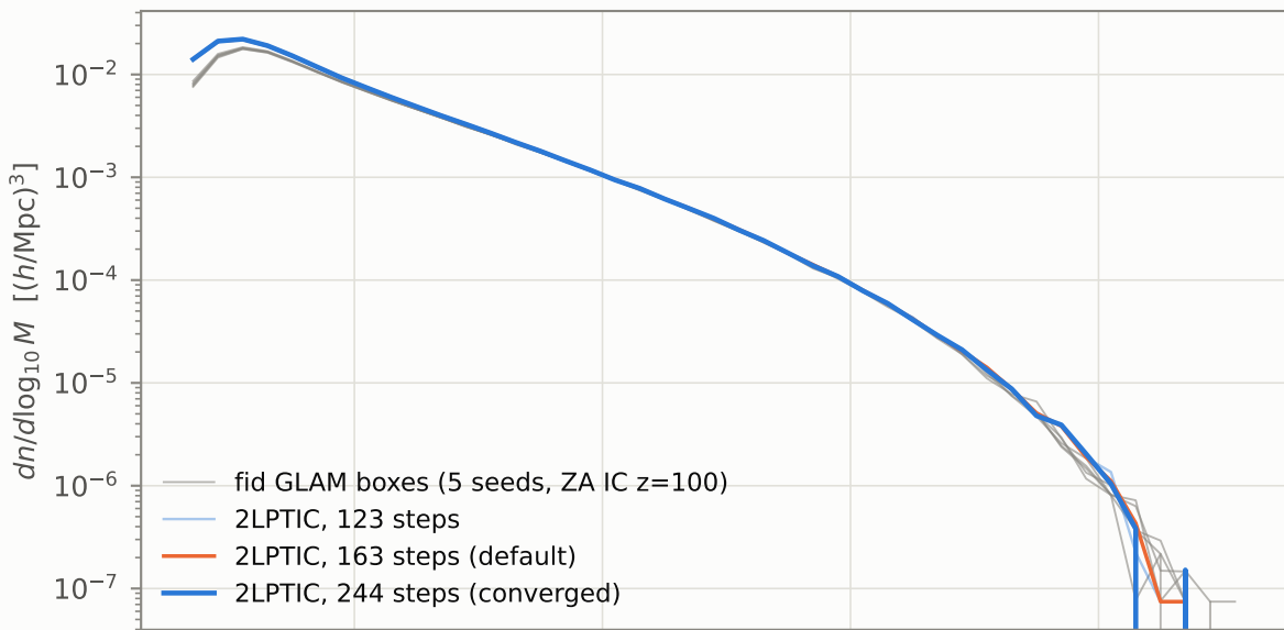
GLAM z = 0 halo mass function: 2LPTIC IC vs the five fiducial boxes BDM M_{\text{tot}} , L = 512 \text{ Mpc}/h , 2048^3 , N_g=4096 ; all interpolated to a = 1
