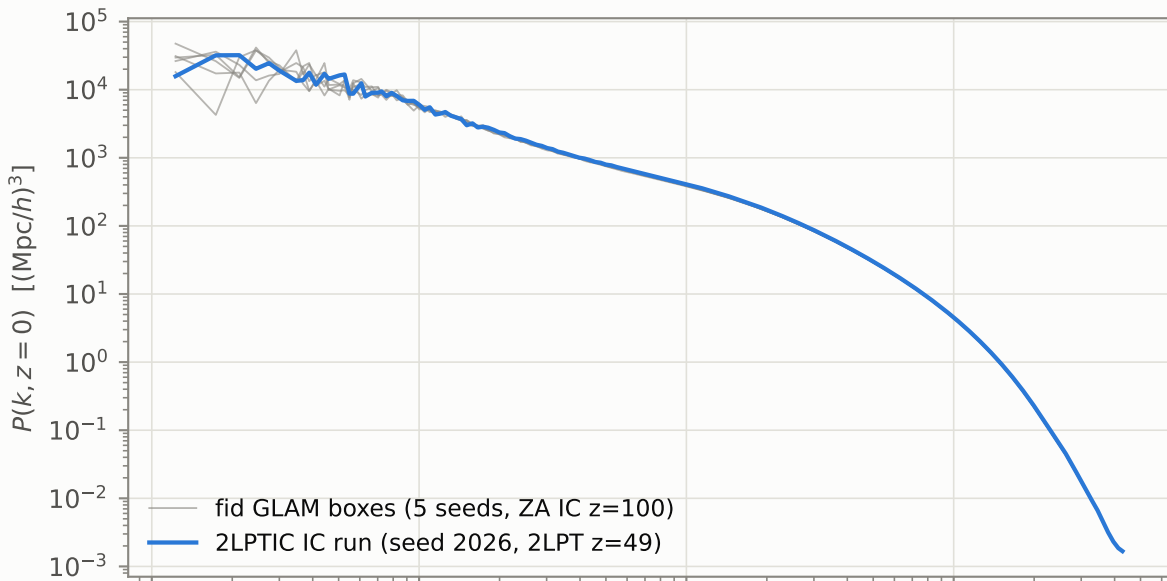
GLAM z = 0 power spectrum: 2LPTIC IC vs the five fiducial boxes L = 512 \text{ Mpc}/h , 2048^3 , N_g=4096 , fid cosmology
