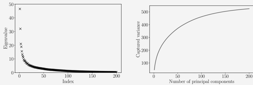
Figure 10.5 Properties of the training data of MNIST “8”. (a) Eigenvalues sorted in descending order; (b) Variance captured by the principal components associated with the largest eigenvalues.
