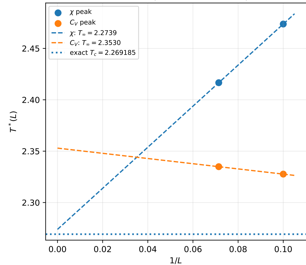
Finite-size shift of pseudocritical temperature
