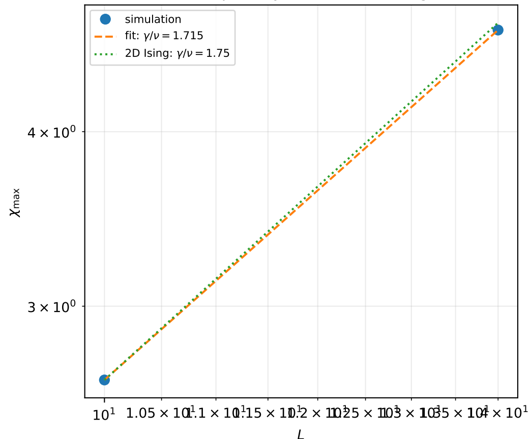
Susceptibility finite-size scaling
