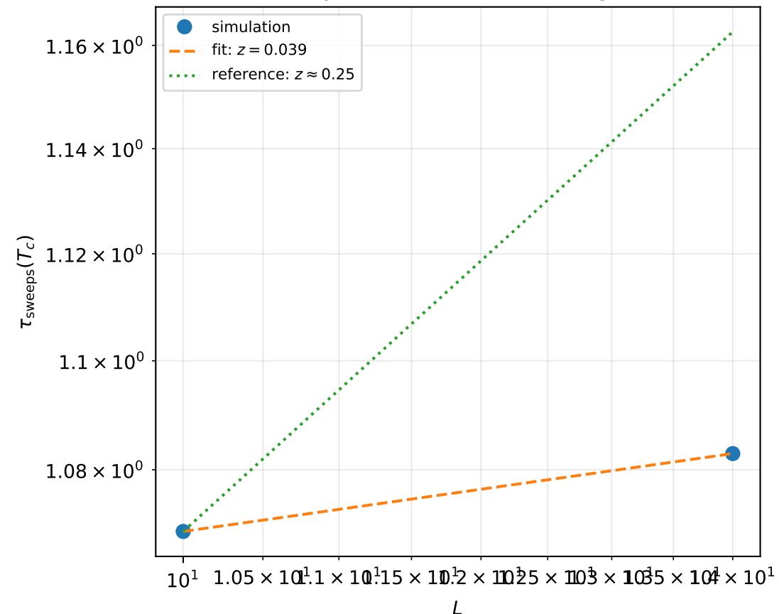
Dynamic finite-size scaling
