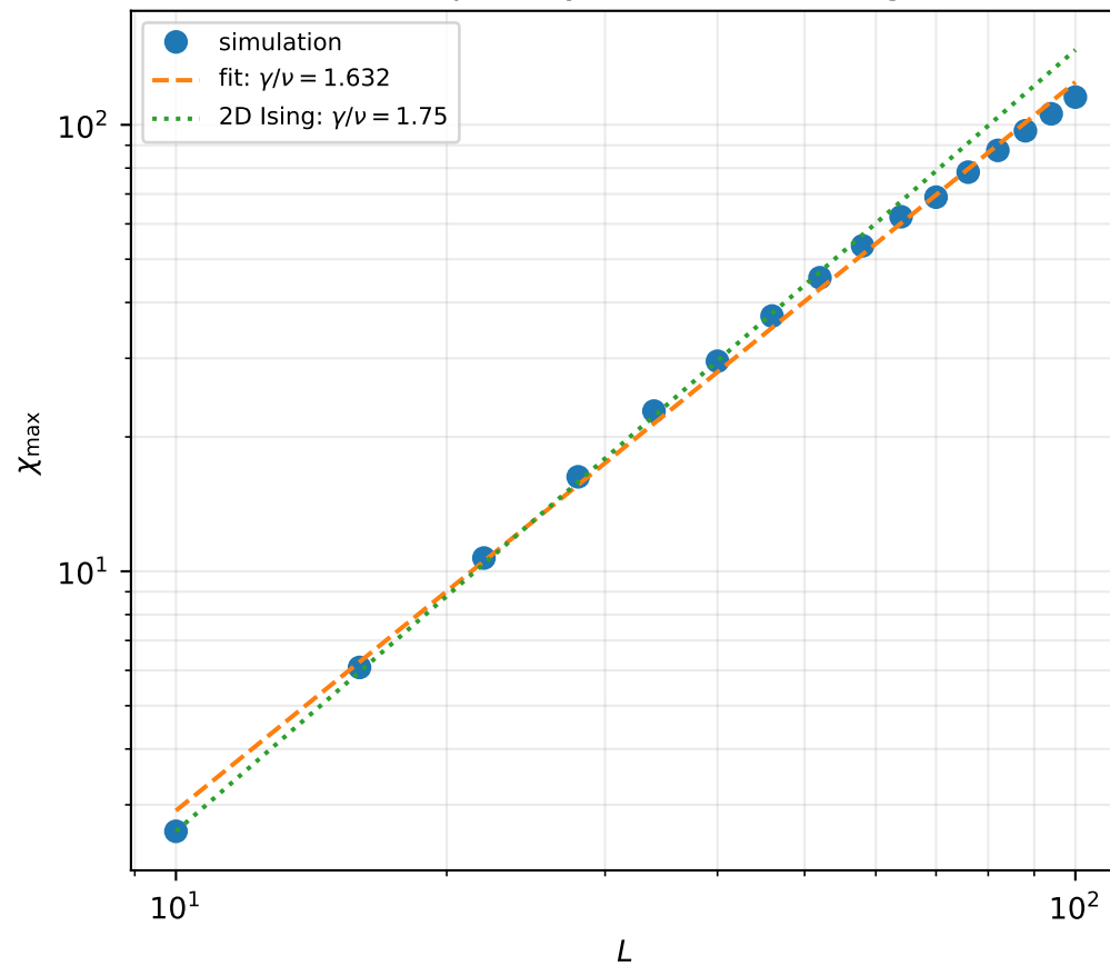
Susceptibility finite-size scaling
