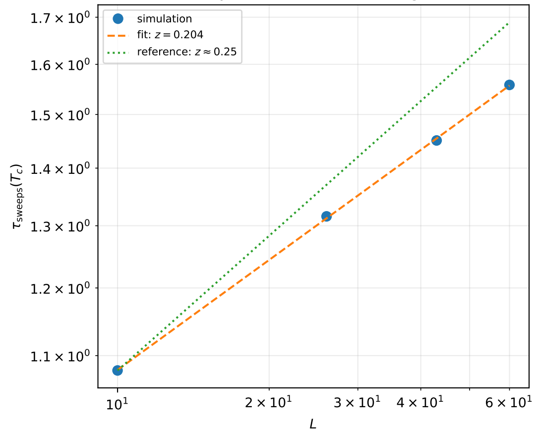
Dynamic finite-size scaling
