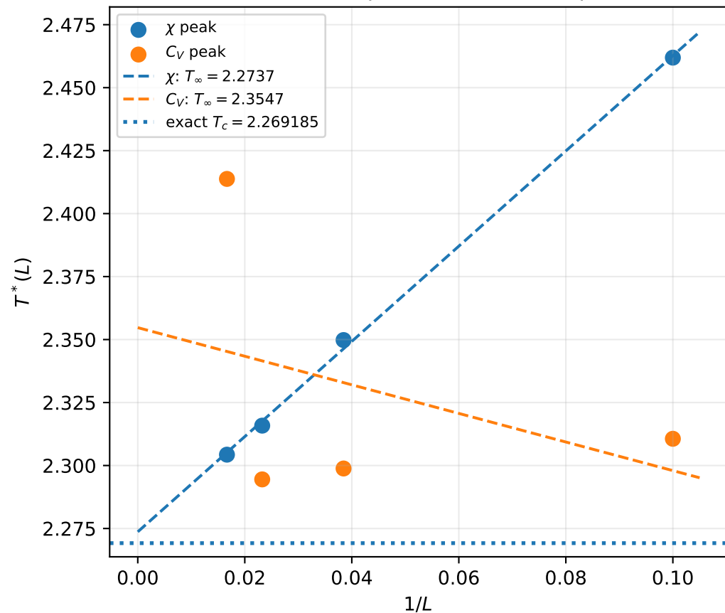
Finite-size shift of pseudocritical temperature
