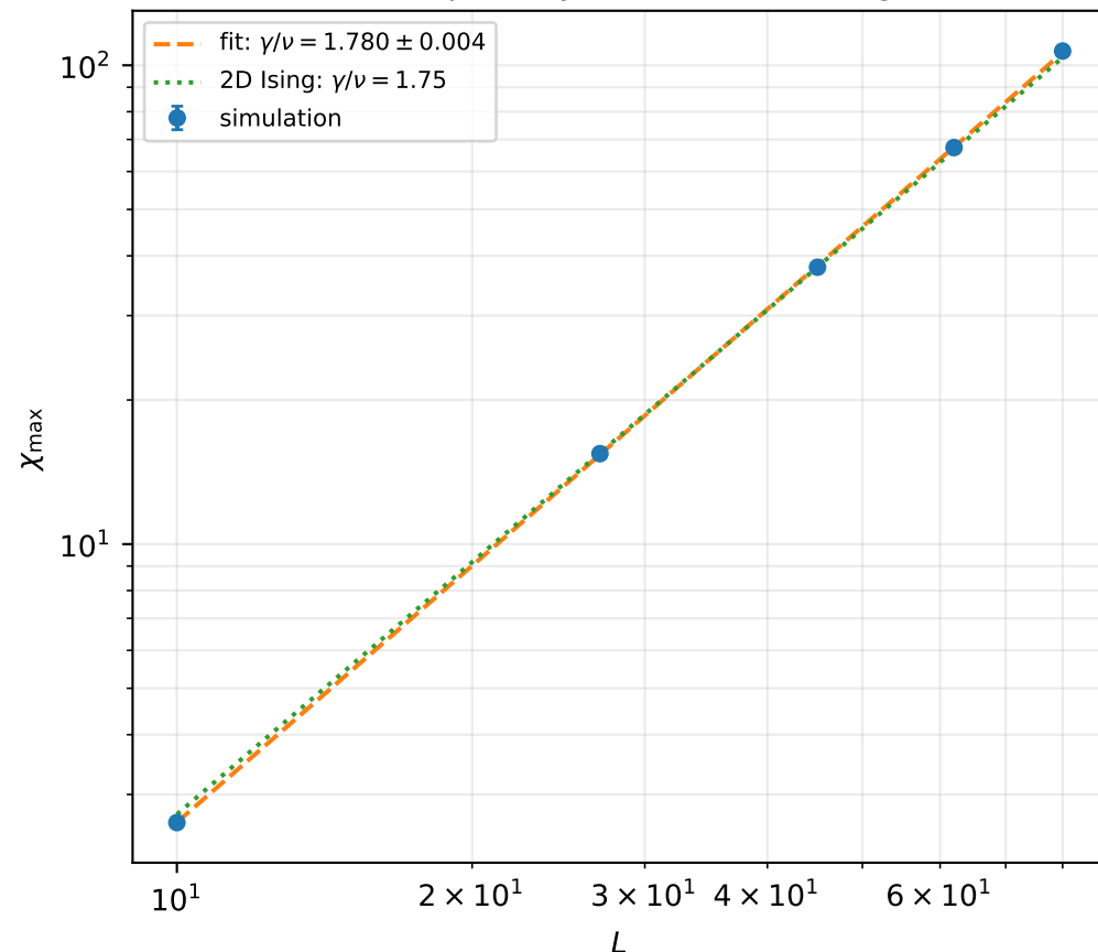
Susceptibility finite-size scaling
