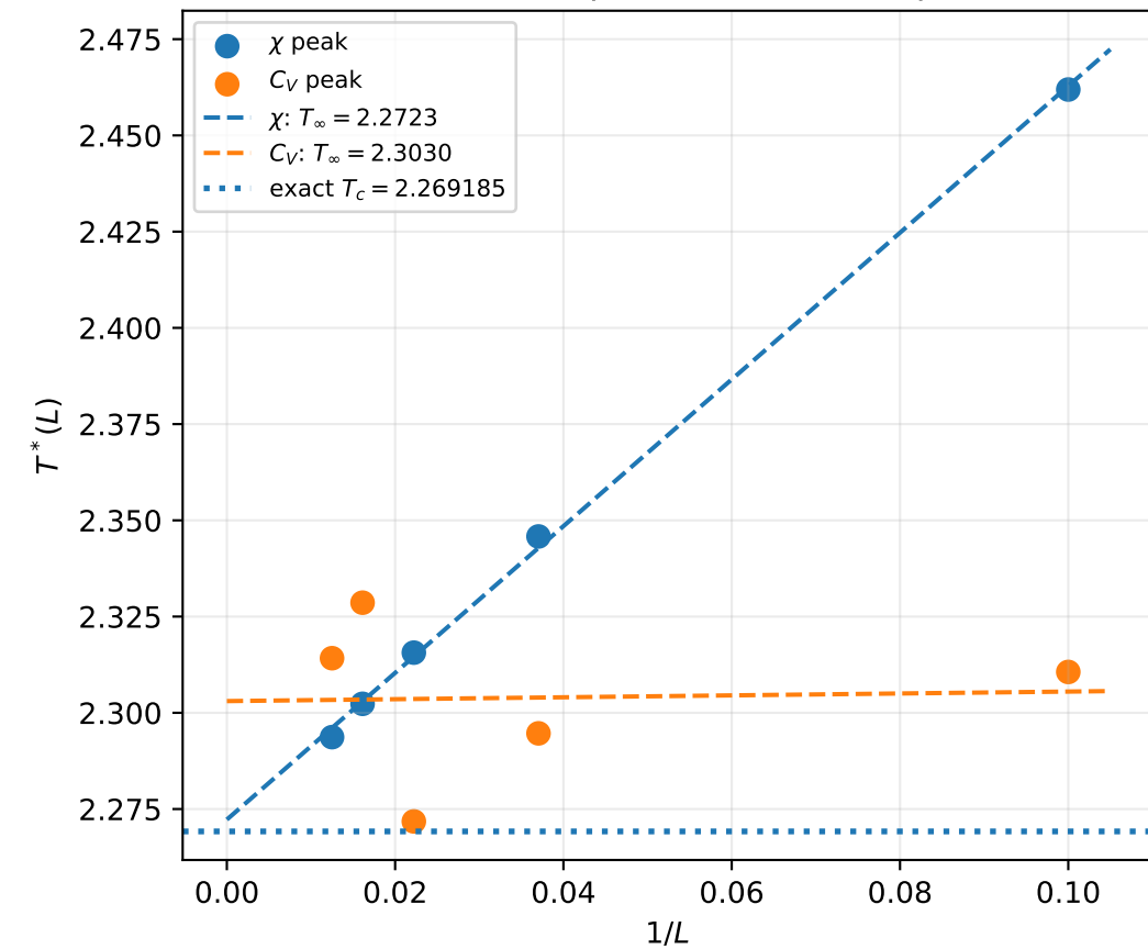
Finite-size shift of pseudocritical temperature
