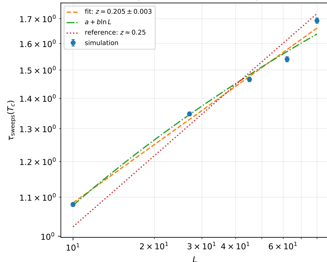
Dynamic finite-size scaling
