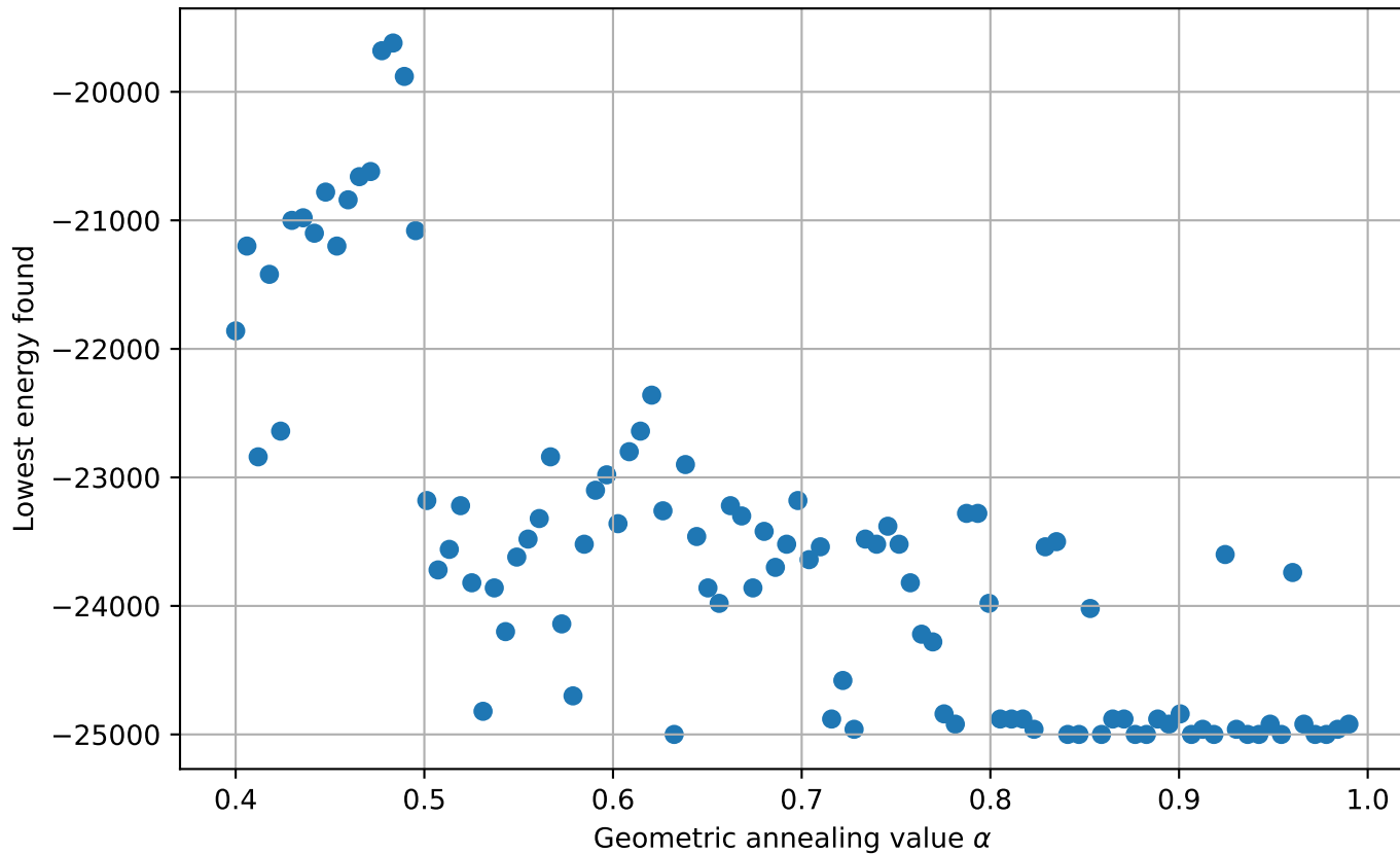
Speed of annealing vs lowest energy found (100 sweeps per Temp)
