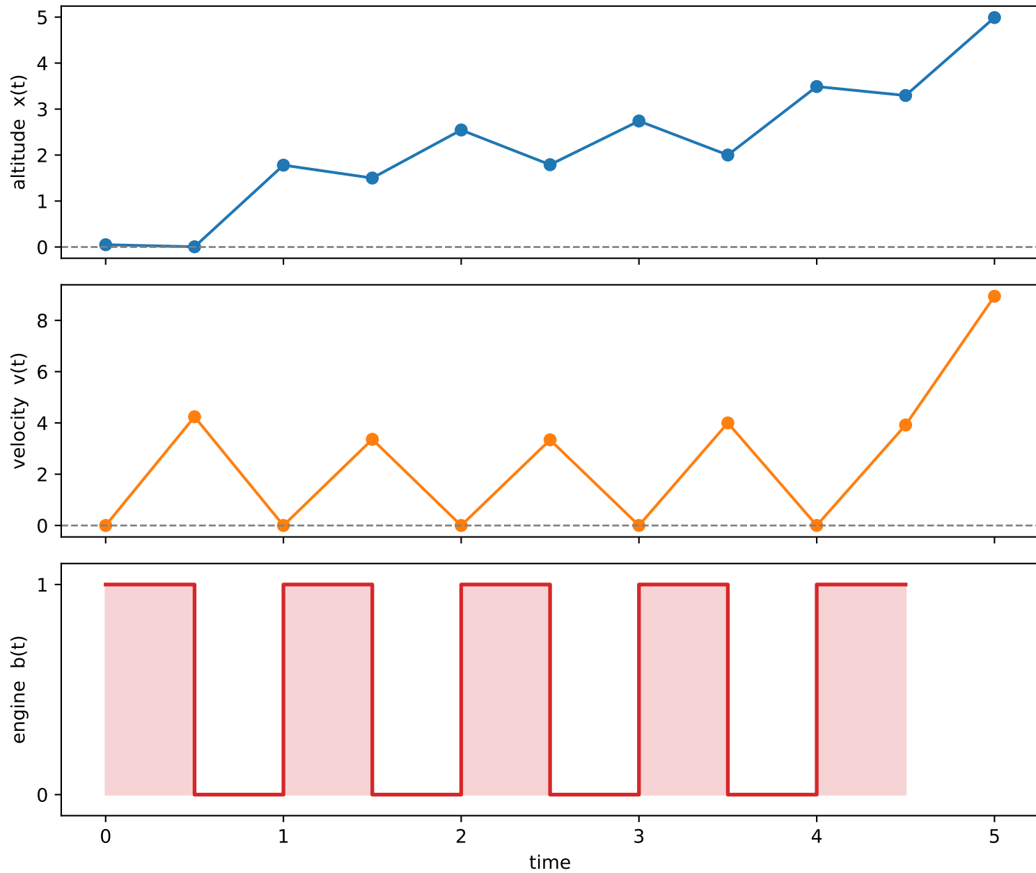
Rocket trajectory
