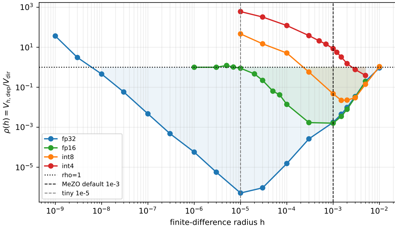
Finite-difference error relative to the random-direction floor
