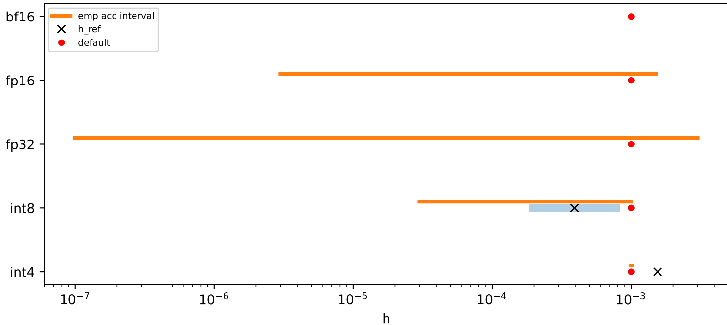
RoBERTa/SST-5 precision windows
