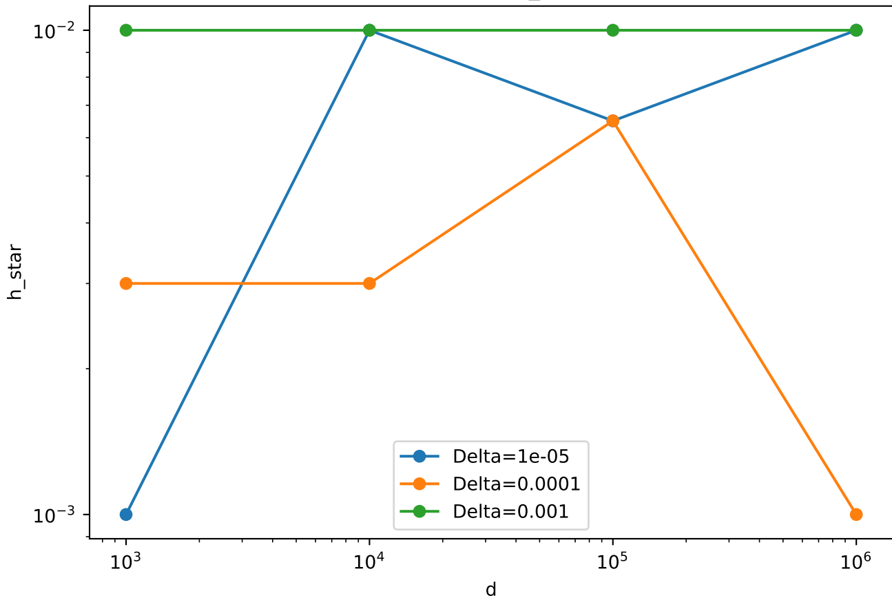
High-dimensional h_{\text{star}} scaling
