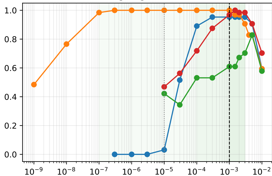
Sign agreement
