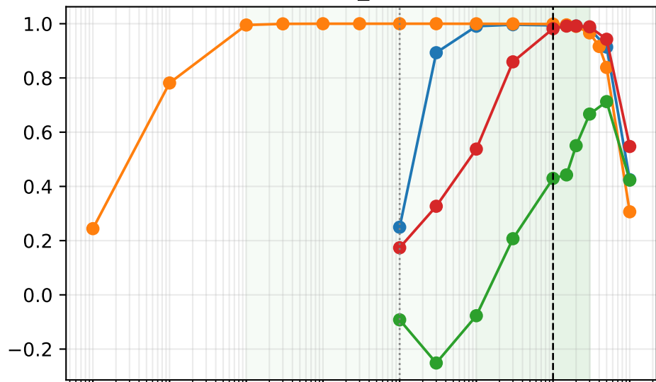
\text{corr}(d_h, d^*)
