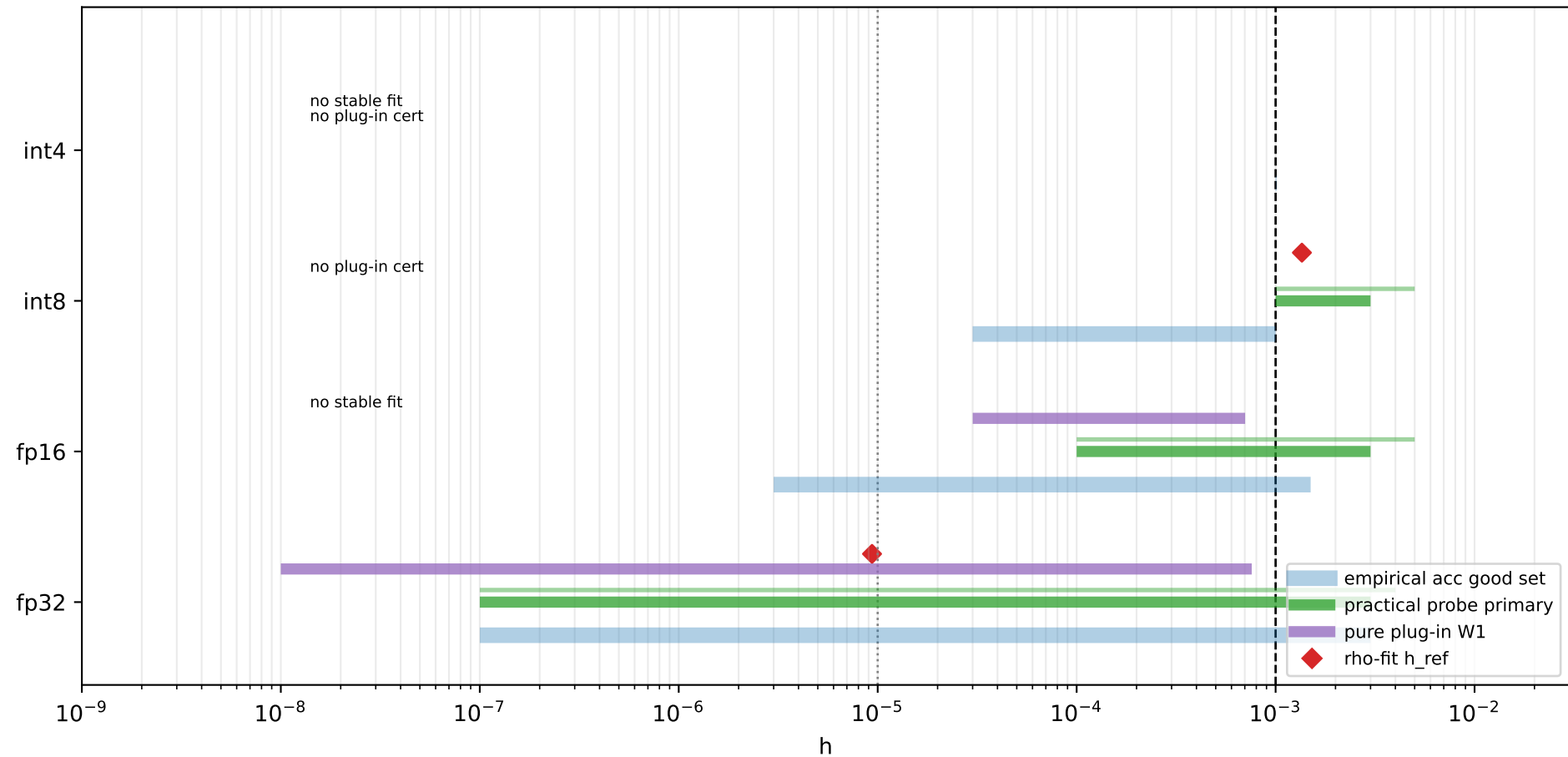
RoBERTa/SST-5 window comparison
