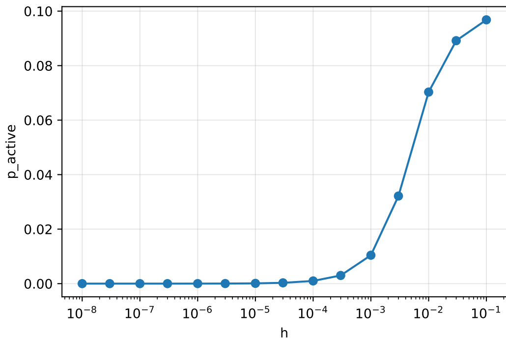
roberta-large / sst-5 / int4 / sparse_p0p1
