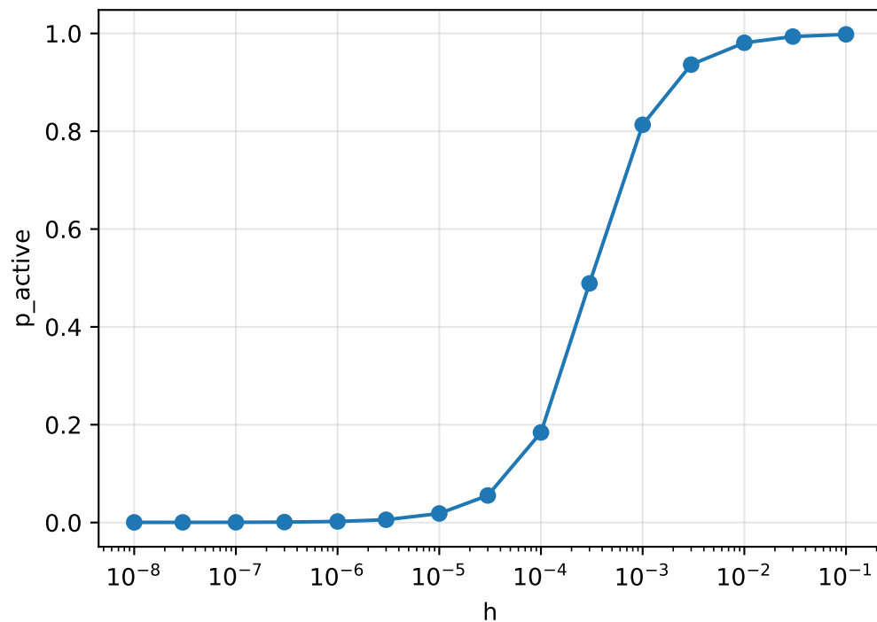
roberta-large / sst-5 / int8 / dense
