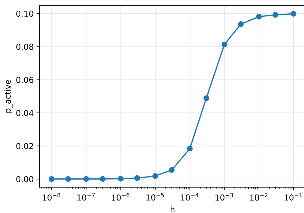
roberta-large / sst-5 / int8 / sparse_p0p1
