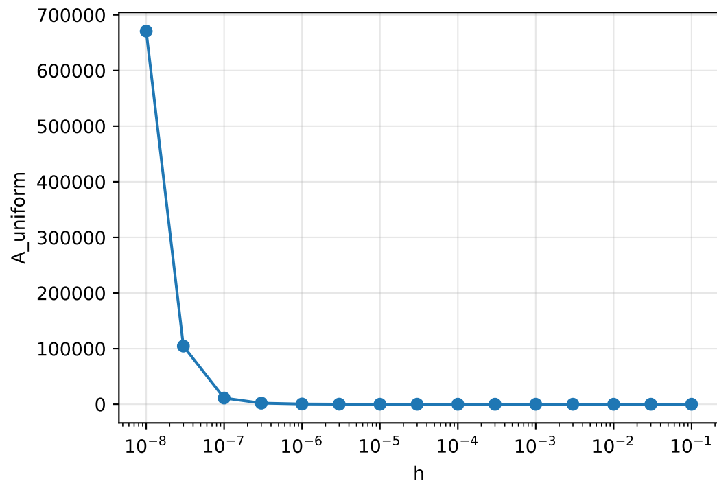
roberta-large / sst-5 / int8 / sparse_p0p1
