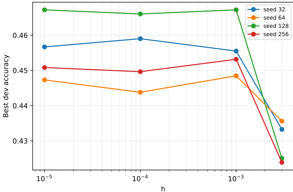
RoBERTa-large / SST-5 FP32 multi-seed plateau
