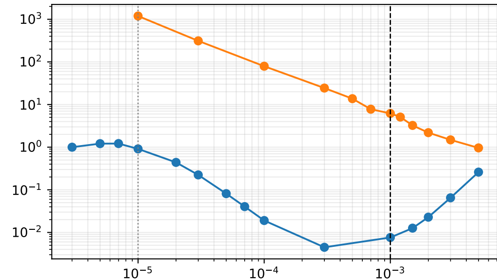
scalar true directional nMSE
