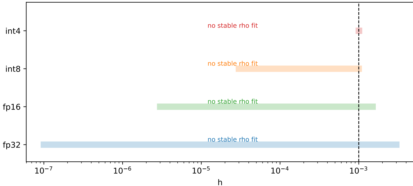
Empirical accuracy good set (light) vs theoretical W1 (dark)
