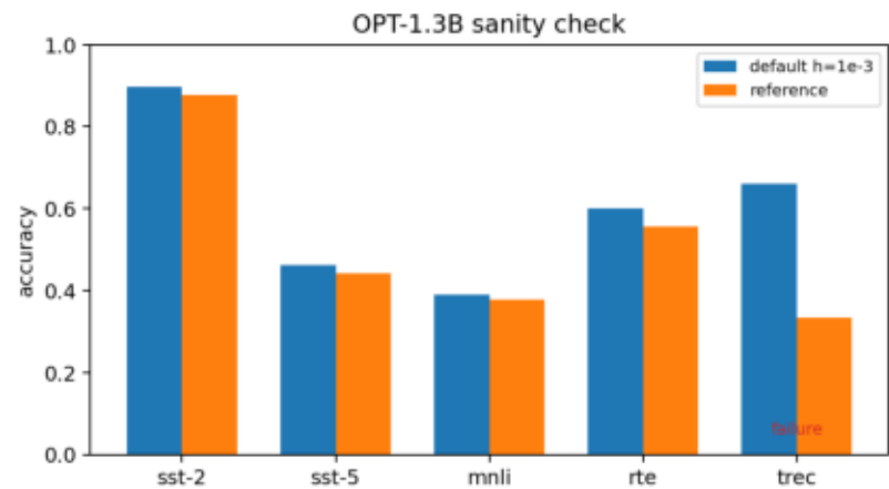
paper_fig_opt_cross_arch.png
