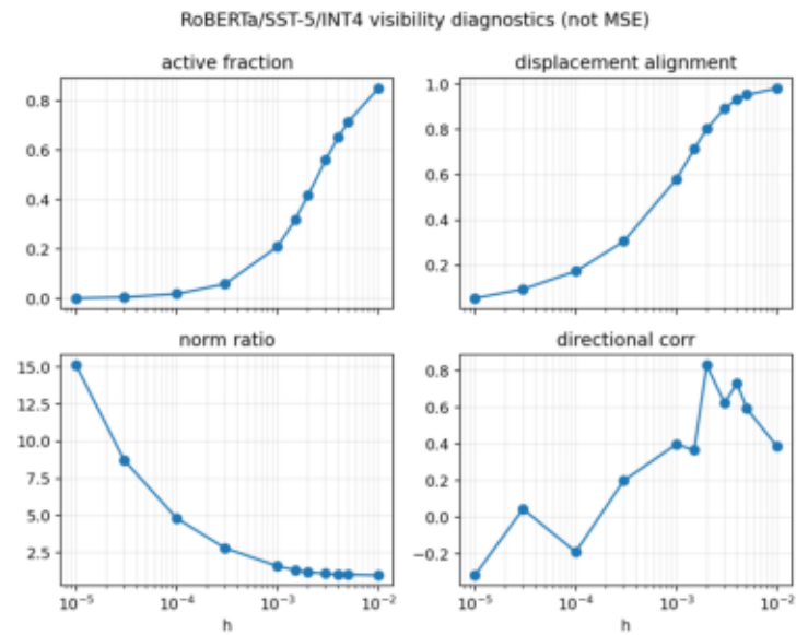
paper_fig_int4_visibility_diagnostics.png
