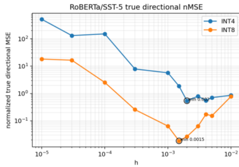
paper_fig_sst5_true_mse.png
