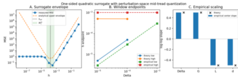
paper_fig_analytic_window.png
