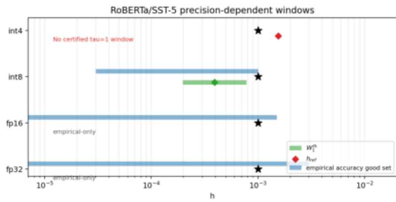
paper_fig_precision_window.png
