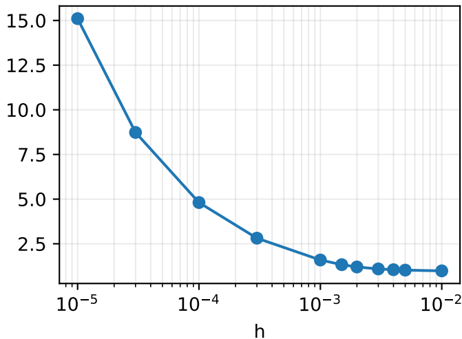
norm ratio
