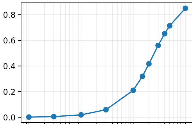
norm ratio
