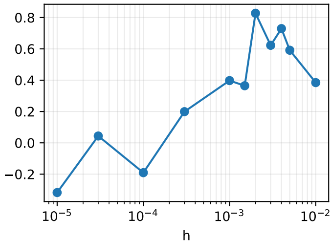
directional corr
