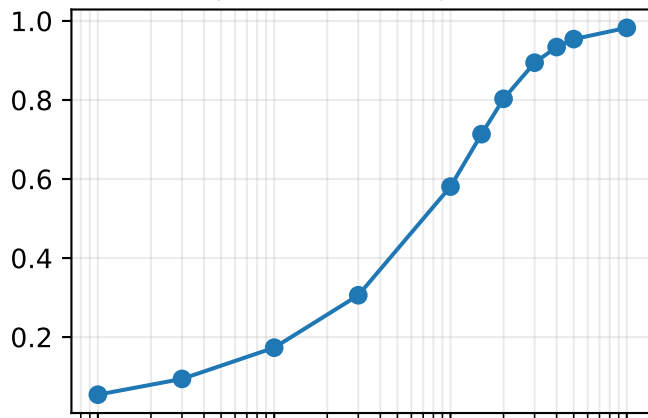
displacement alignment
