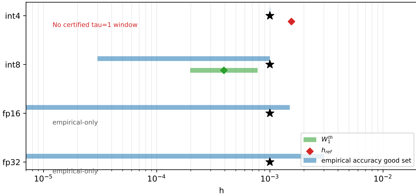
RoBERTa/SST-5 precision-dependent windows
