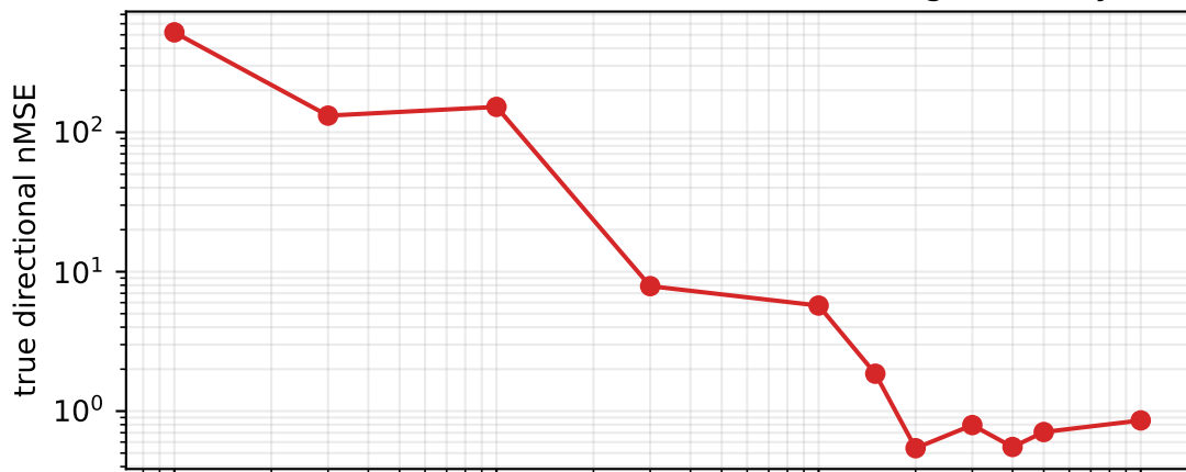
RoBERTa/SST-5/INT4 true MSE and training accuracy
