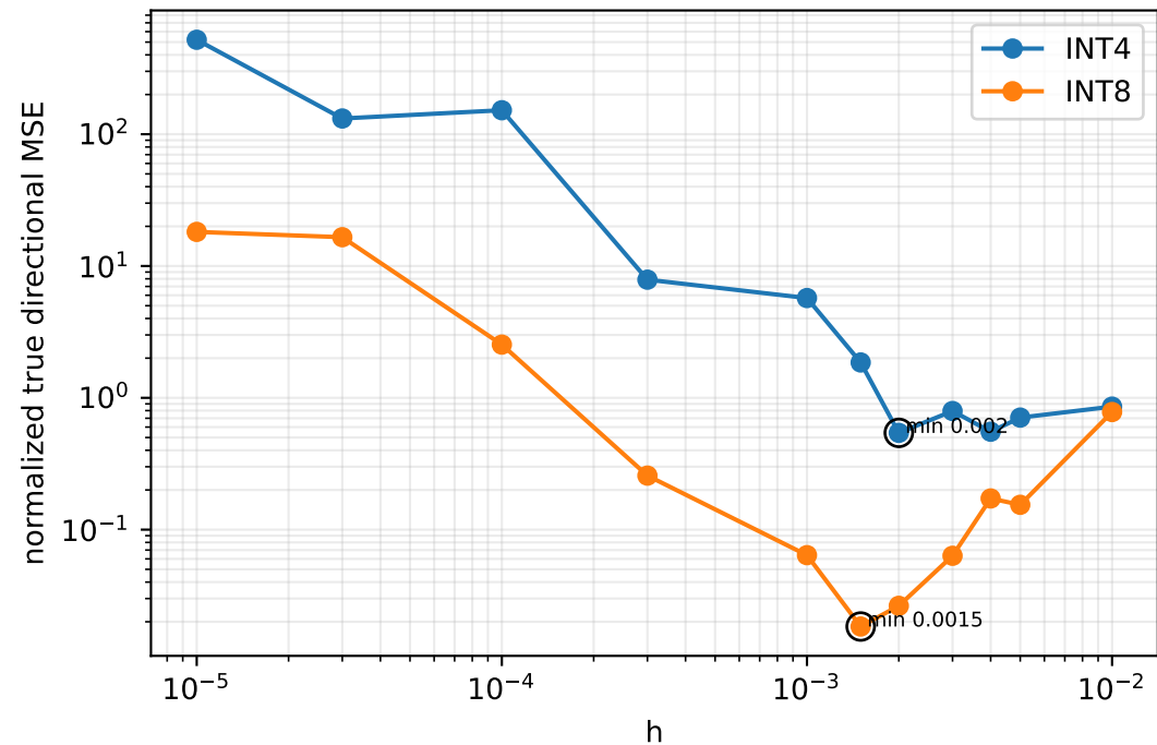
RoBERTa/SST-5 true directional nMSE
