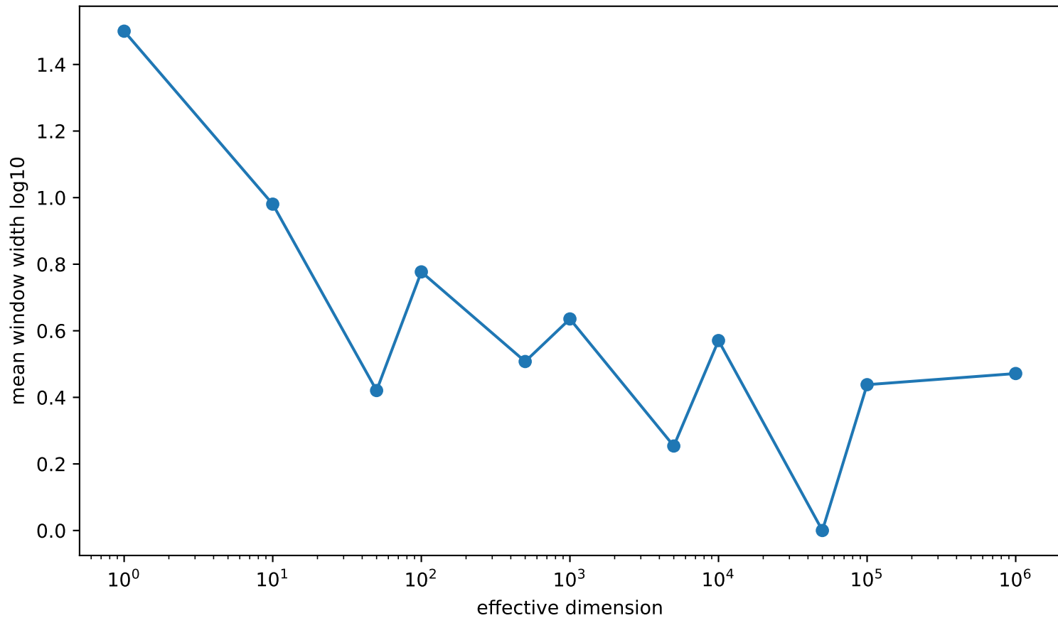
Synthetic effective dimension vs window width
