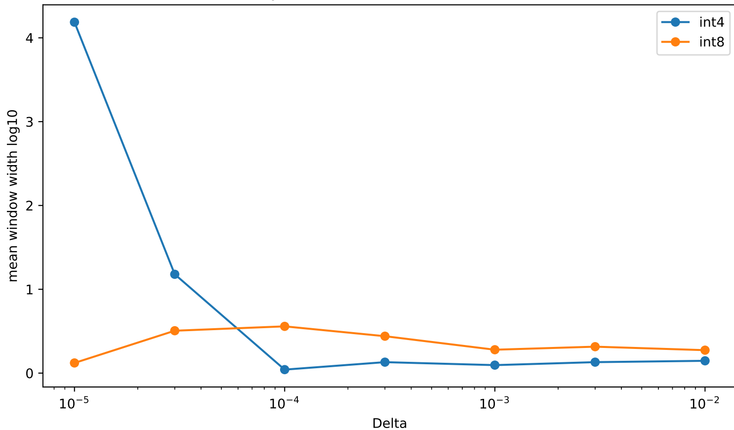
Synthetic window width vs Delta
