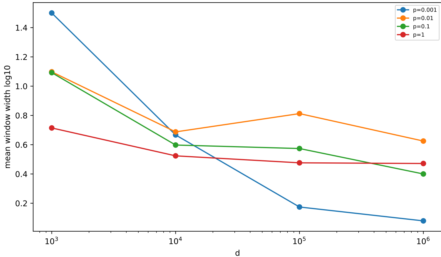
Synthetic window width vs dimension
