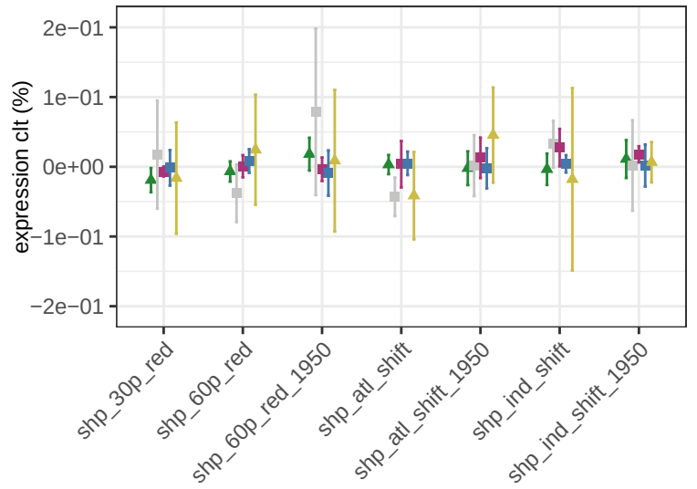
total cloud cover percentage – NH-land
