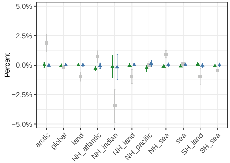
cloud cover percentage – shp-60p-red
