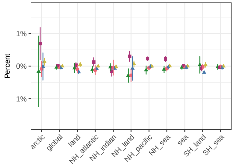
Dimethyl sulphide (DMS) mole fraction – shp-60p-red
