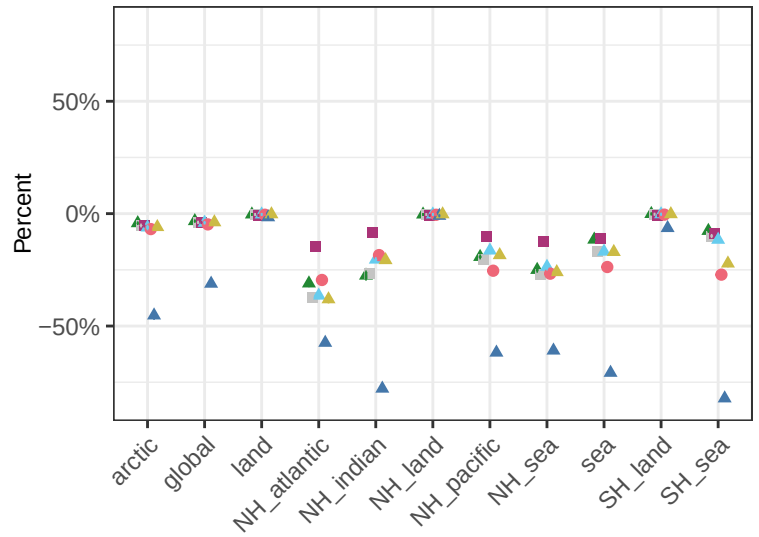
surface concentration of SO4 – shp-60p-red
