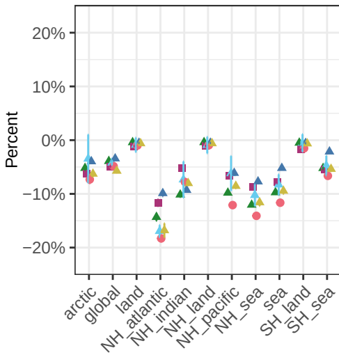
wet deposition rate of so4 – shp-60p-red
