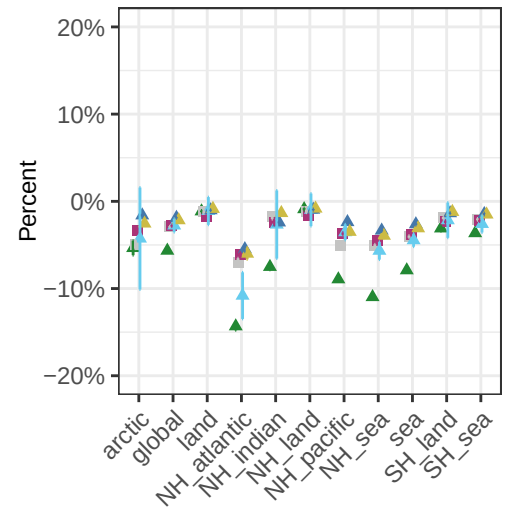
dry deposition rate of so4 – shp-60p-red
