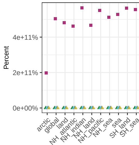
total deposition rate of S – shp-60p-red
