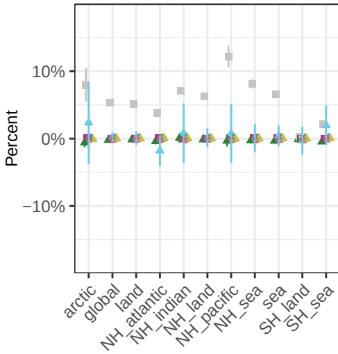
dry deposition rate of so2 – shp-60p-red
