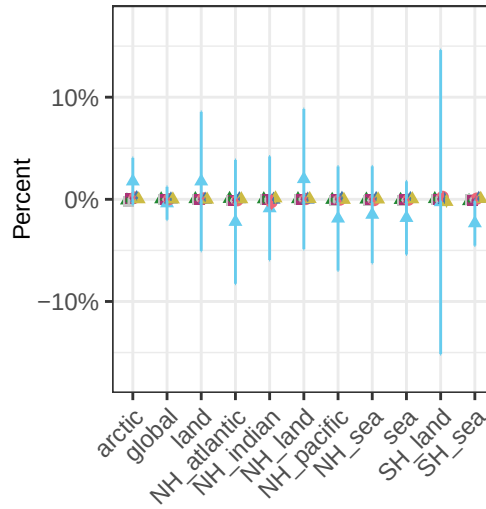
wet deposition rate of so2 – shp-60p-red
