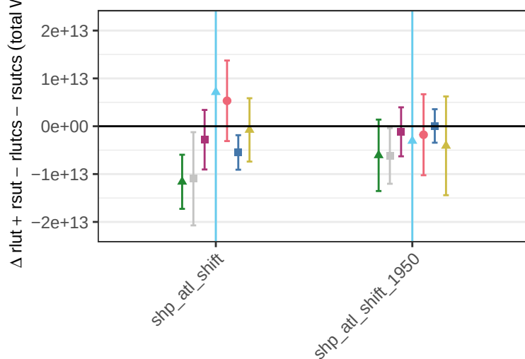
implied cloud response at TOA - [Atlantic] - [Pacific]
