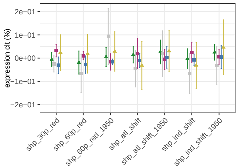
total cloud cover percentage – NH-atlantic
