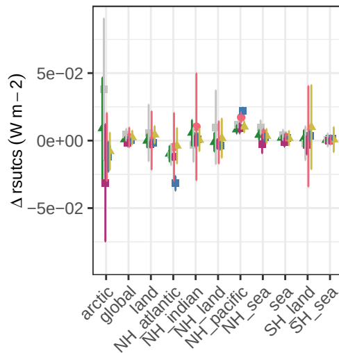
upwelling clear-sky shortwave flux flux at TOA – shp-atl-shift-1950
