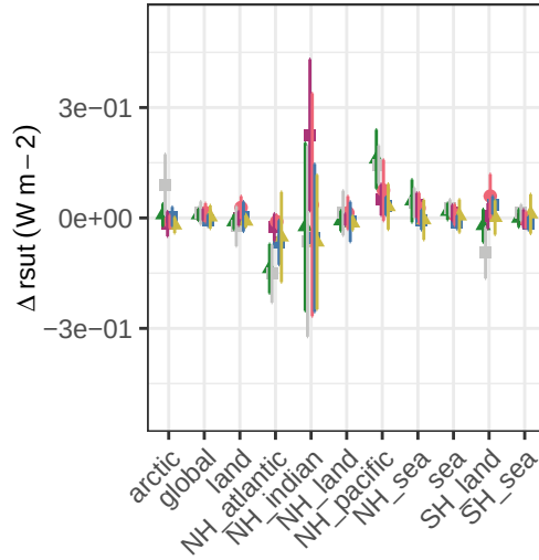
implied cloud response at TOA – shp-atl-shift-1950
