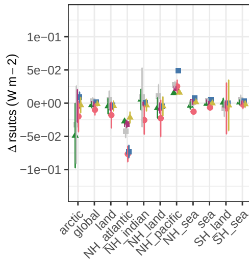
upwelling clear-sky shortwave flux at TOA – shp-atl-shift
