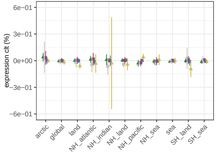
cloud cover percentage – shp-atl-shift
