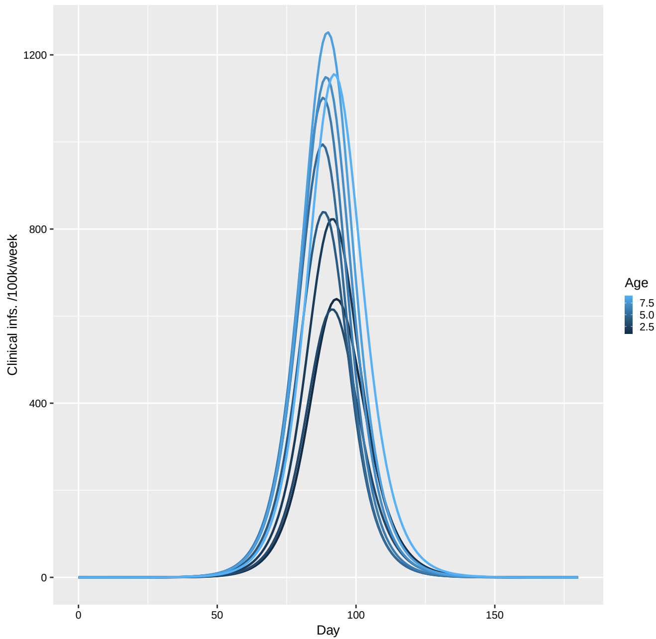
COVID-19, Urban
