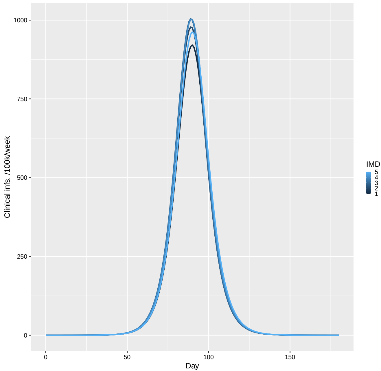
COVID-19, Urban
