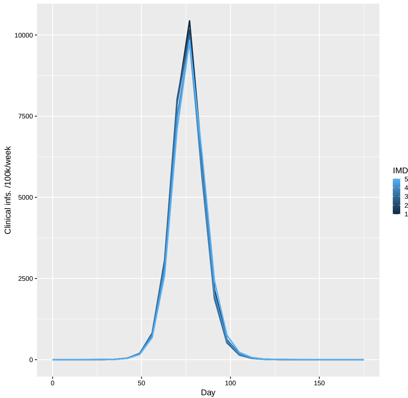
RSV-illness, Urban by SE strata
